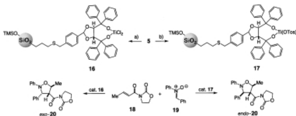
Scheme 6. Preparation of the heterogeneous Ti-TADDOLates 16 and 17 and their use in the 1,3-dipolar cycloaddition of crotonoyloxazolidinone 18 to diphenyl nitrene 19 to give either exo - 20 (using the titanate 16 ) or endo - 20 (using the titanate 17 ). [47] For the results concerning conversion and stereoselectivities, see Figures 6 and 7, respectively. a) \text{TiCl}_2(\text{OiPr})_2 , toluene, azeotropic removal of the i PrOH formed; b) \text{Ti}(\text{OTos})_2(\text{OiPr})_2 , toluene, azeotropic removal of the i PrOH formed.
