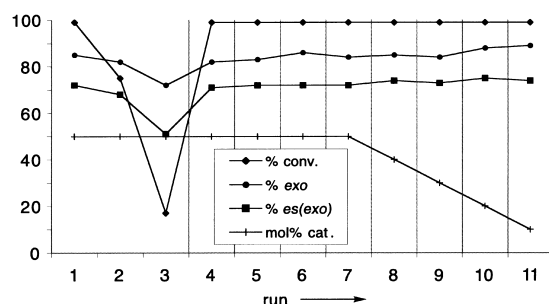
Figure 6. 1,3-Dipolar cycloaddition of nitrene 19 to the crotonoyl double bond of compound 18 (Scheme 6) using variable amounts of the heterogeneous \text{Cl}_2\text{Ti} -TADDOLate 16 . A vertical bar between two runs stands for a \text{HCl}/\text{H}_2\text{O} /acetone hydrolysis step with subsequent reloading by titanate between these corresponding two runs.
