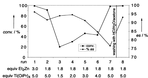
Figure 3. Results of the addition of \text{Et}_2\text{Zn} to \text{PhCHO} in the presence of a hydrophilic analogue of silica gel 5 (made by grafting of a suitable benzyl bromide-substituted TADDOL on silica gel 1 ). The curve showing the conversion belongs to the left y axis and the curve showing the enantioselectivity belongs to the right y axis with a different scale!
