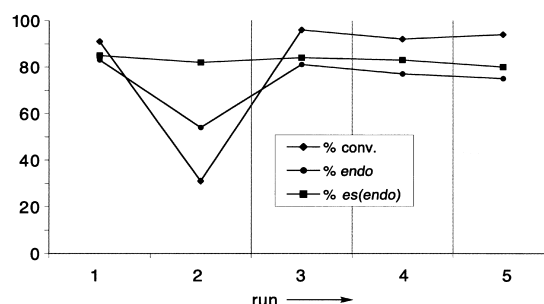
Figure 7. 1,3-Dipolar cycloaddition ( 18 + 19 ) (Scheme 6) mediated by the heterogeneous (\text{Tos})_2\text{Ti} -TADDOLate 17 . A vertical bar between two runs indicates a \text{HCl}/\text{H}_2\text{O} /acetone washing step, with subsequent reloading with titanate between these two runs.
